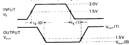
Test Circuit for t_f(0) and t_f(1) .
