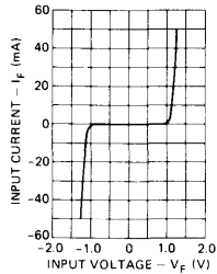
FIGURE 1. INPUT CHARACTERISTICS
