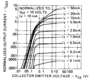
FIGURE 2. TRANSFER CHARACTERISTICS
