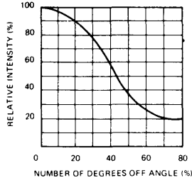
RELATIVE LUMINOUS INTENSITY VS ANGLE
