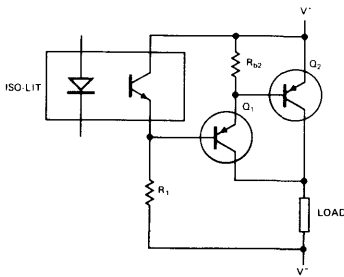
Figure 6B. PNP Darlington HV Booster
