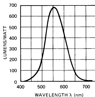
Figure 2. CIE standard photopic luminosity function.
